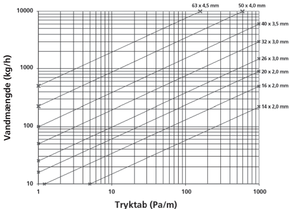
Tryktabsdiagram for Roth Alu-LaserPlus® rør
